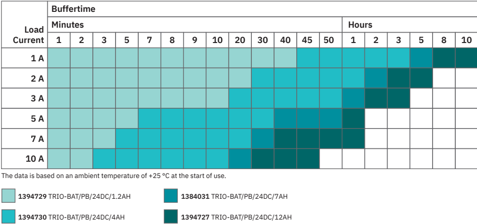
TRIO battery buffer times for TRIO3 UPS
