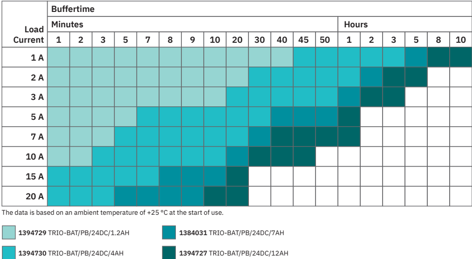
TRIO battery buffer times for TRIO UPS 2G
