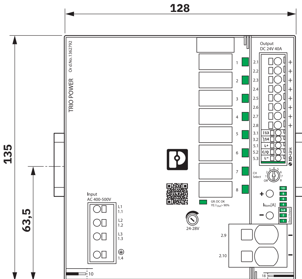
Dimensional drawing
