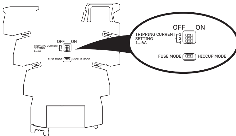
Functional drawing
