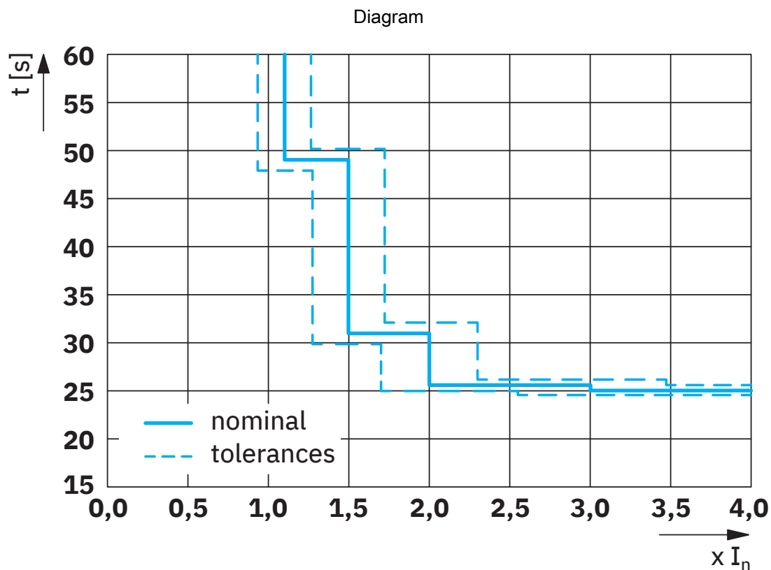
Tripping characteristics in HICCUP MODE
