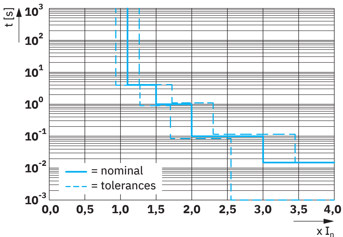
Tripping characteristics in FUSE MODE
