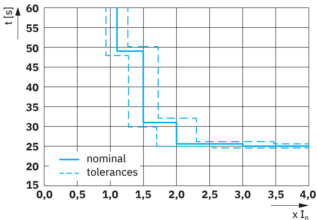
Tripping characteristics in HICCUP MODE
