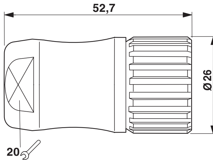
Dimensional drawing
