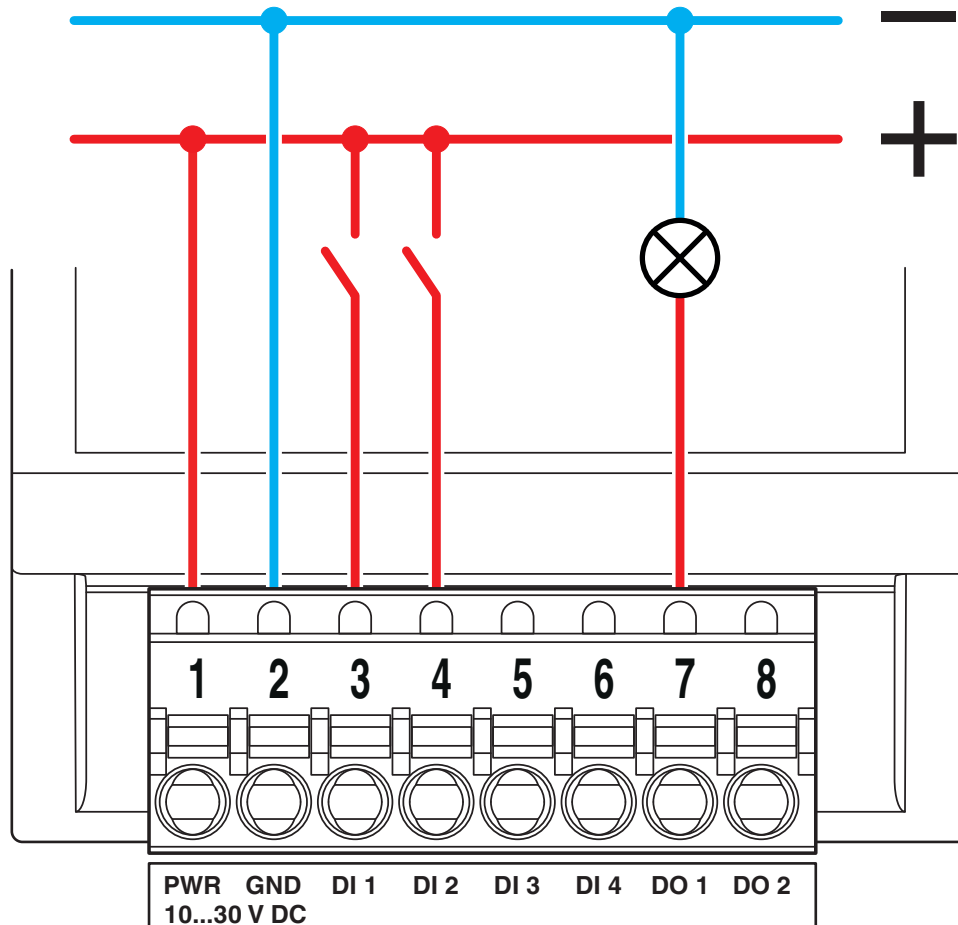
Connection diagram
