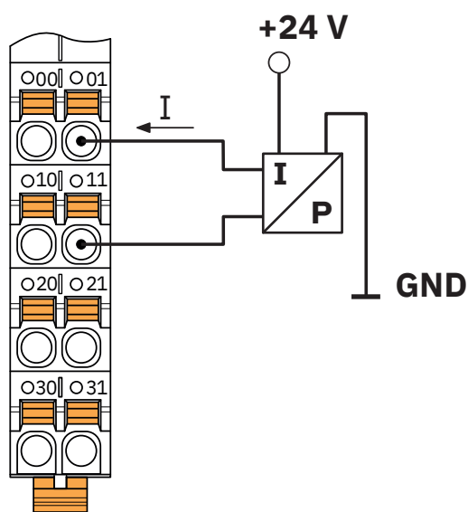
Connection diagram
