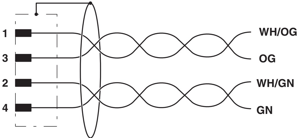
Circuit diagram
