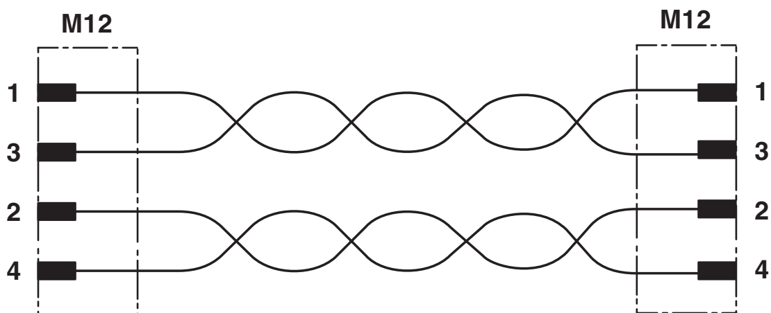
Contact assignment of M12 connector/socket
