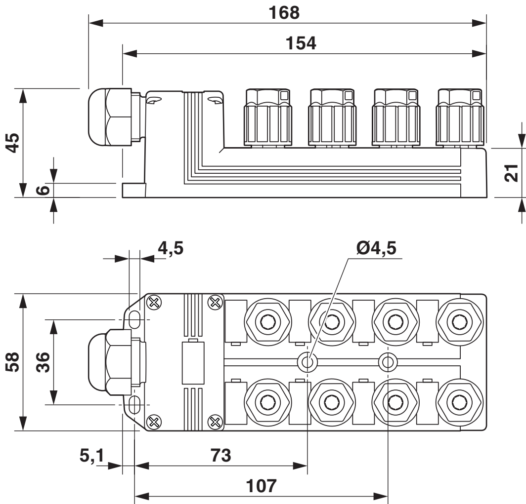
Dimensional drawing
