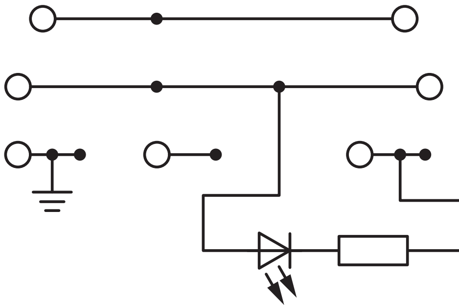
Circuit diagram
