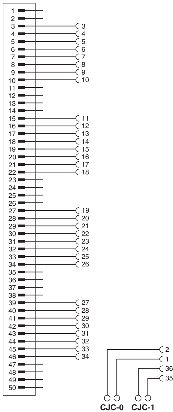
Circuit diagram
