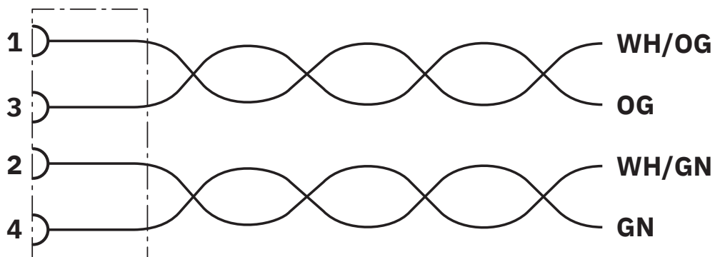
Circuit diagram
