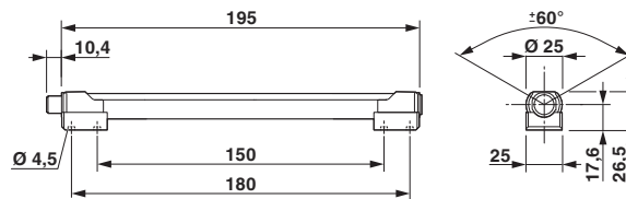
Dimensional drawing
