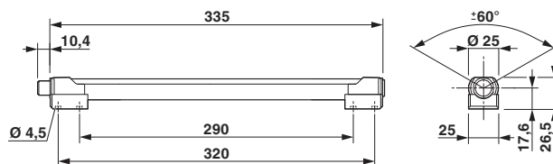
Dimensional drawing
