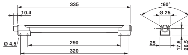
Dimensional drawing
