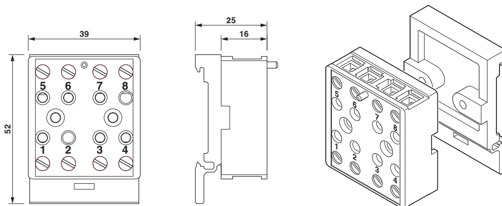
Dimensional drawing
