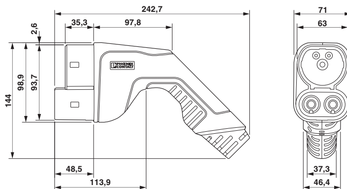
Dimensional drawing
