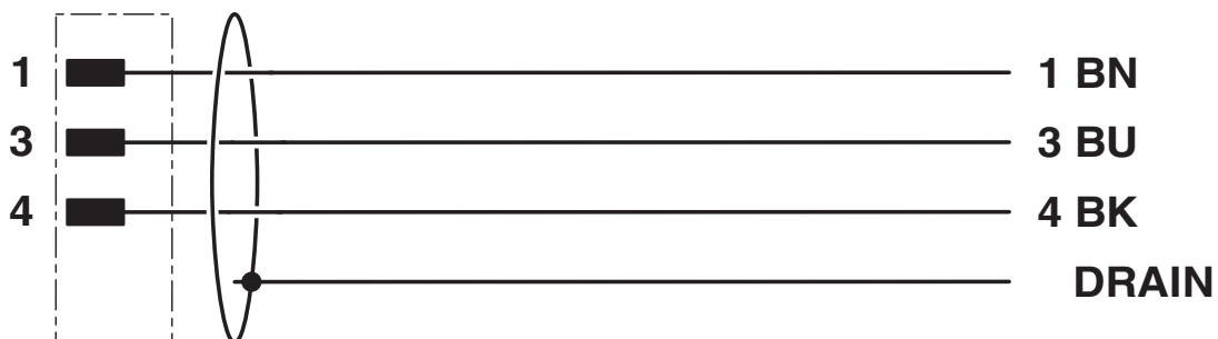
Contact assignment of the M12 plug
