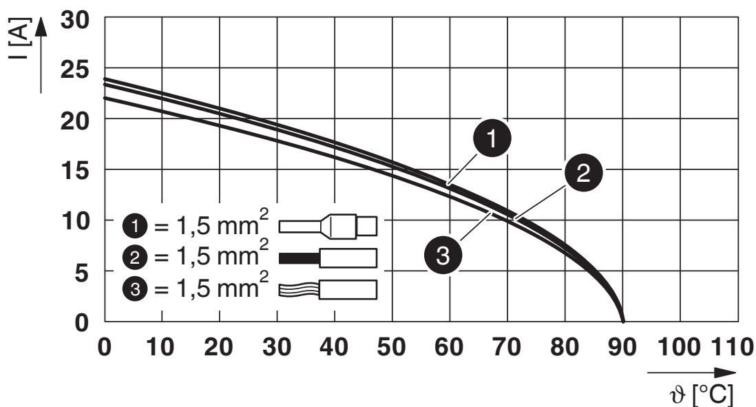
Derating diagram for 1.5 mm 2
