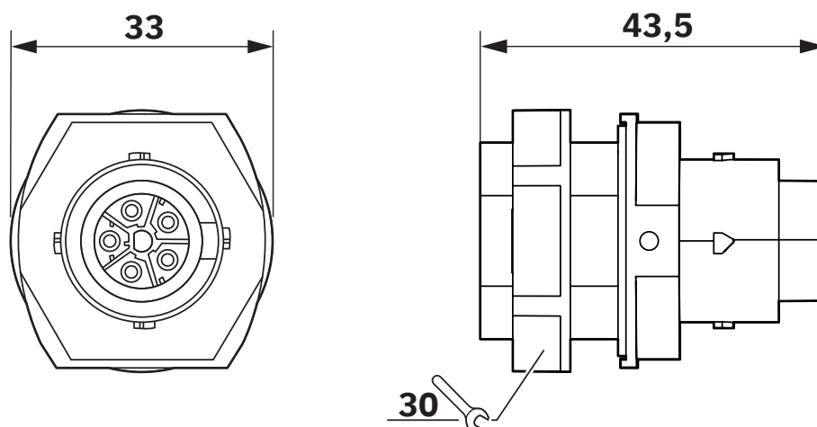
Dimensional drawing
