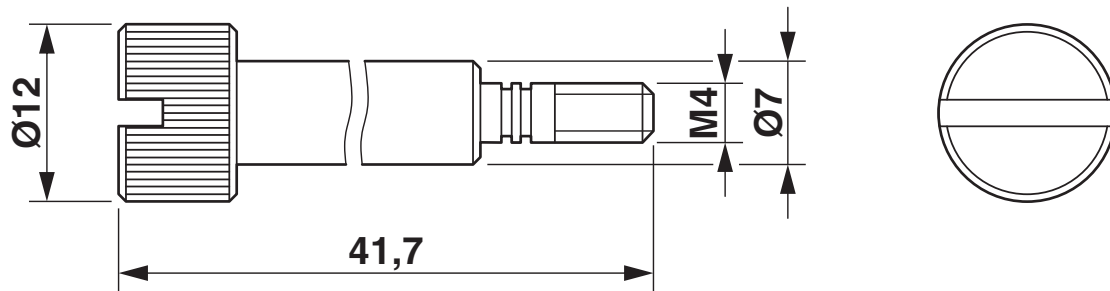
Dimensional drawing
