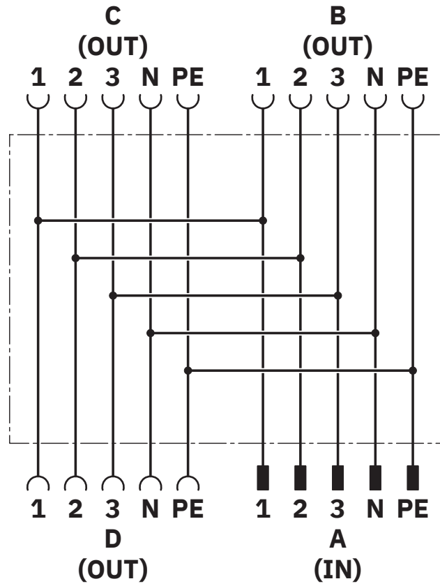
Circuit diagram
