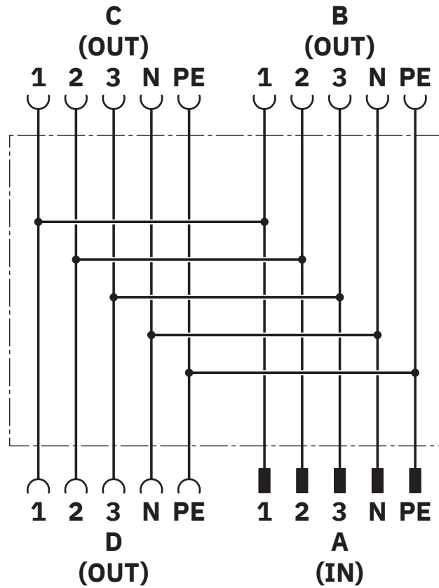
Circuit diagram
