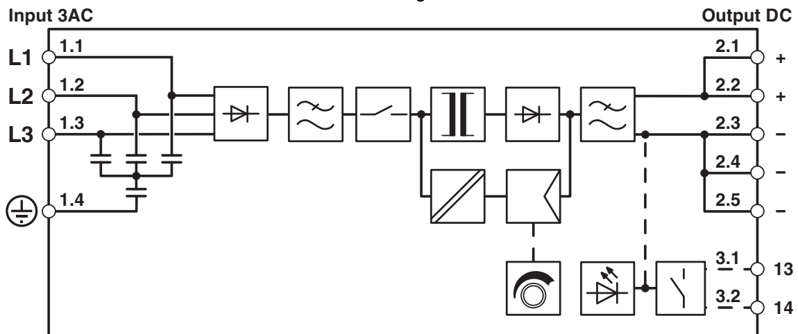
Block diagram
