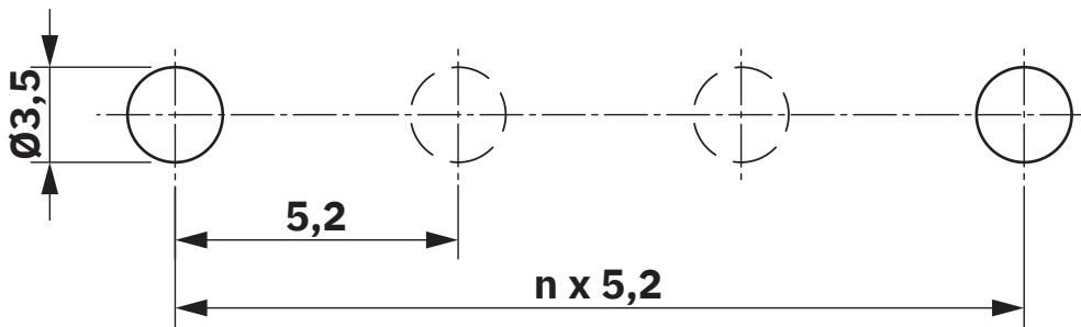
Dimensional drawing
