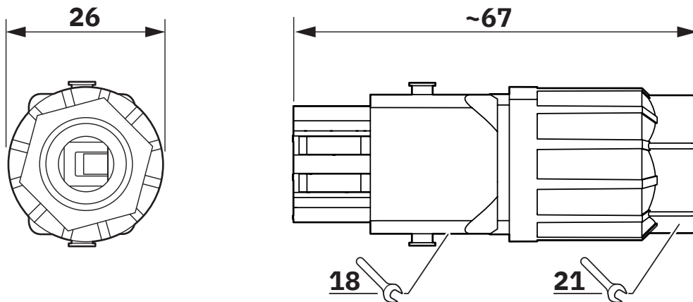
Dimensional drawing
