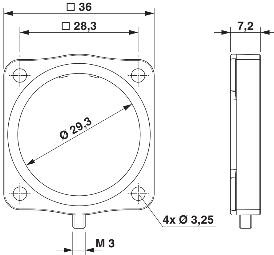
Dimensional drawing
