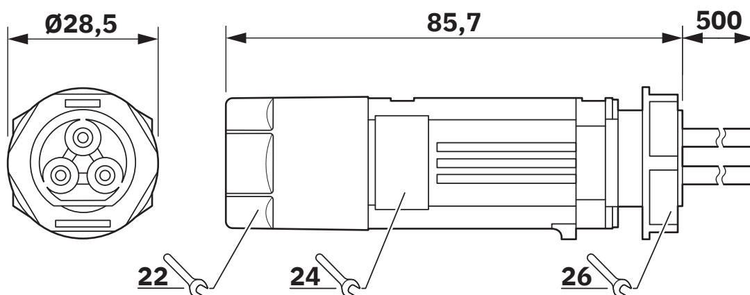
Dimensional drawing
