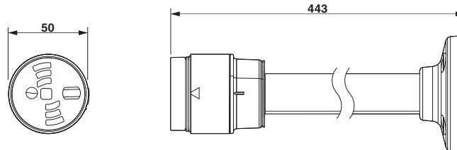
Dimensional drawing
