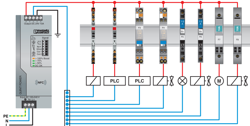
Application drawing
