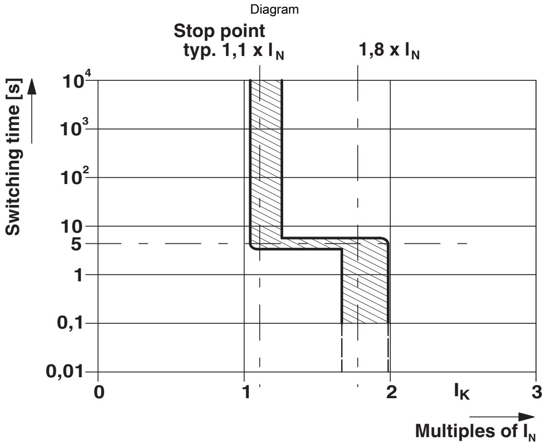
Trigger characteristic
