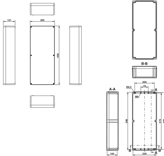
Dimensional drawing
