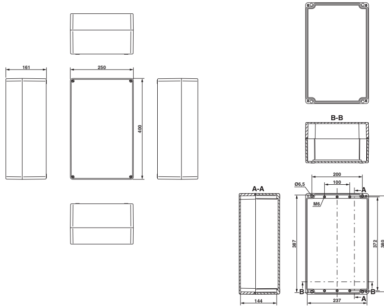
Dimensional drawing
