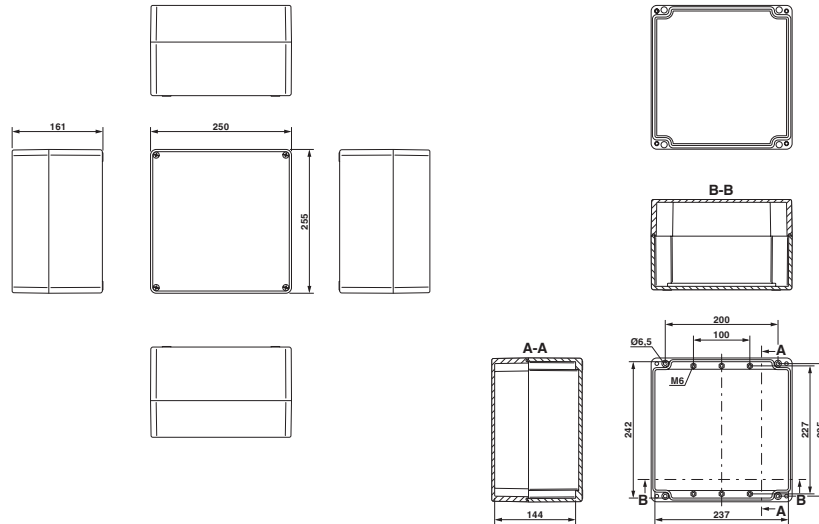
Dimensional drawing
