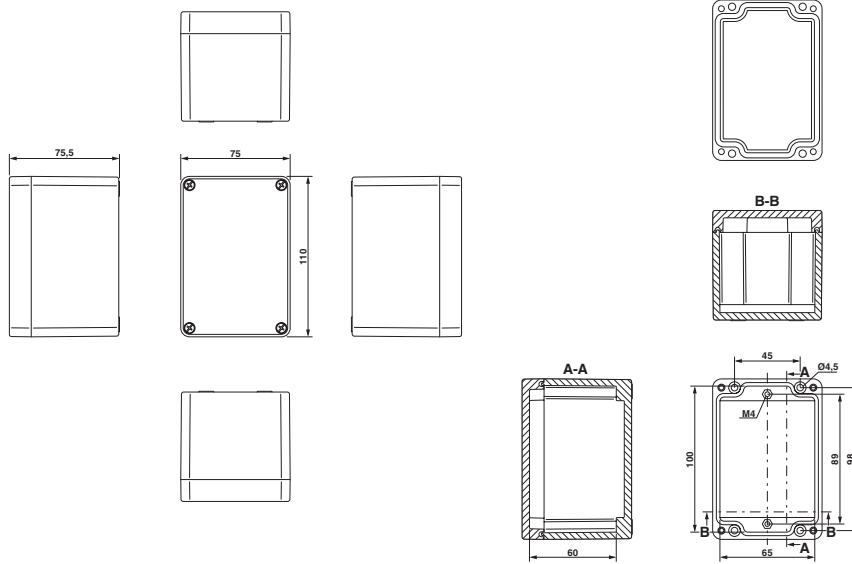
Dimensional drawing
