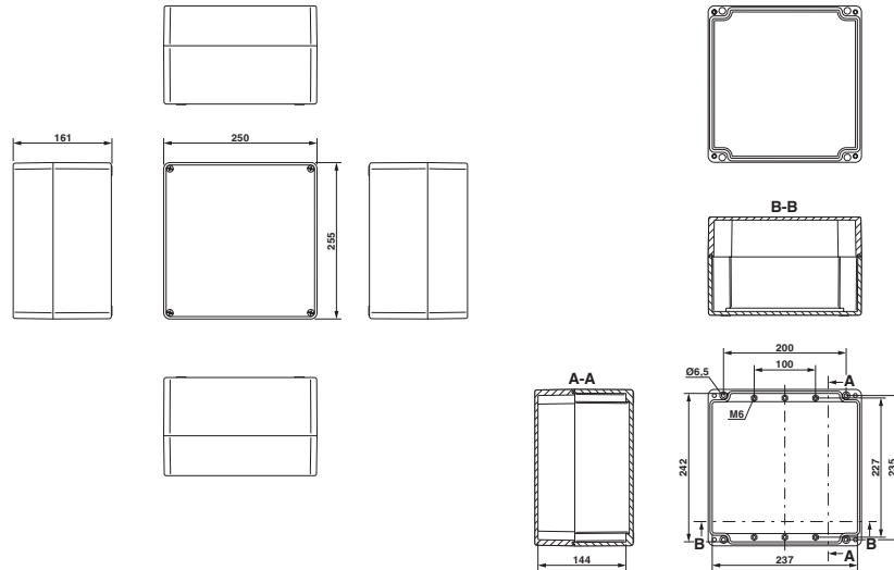
Dimensional drawing
