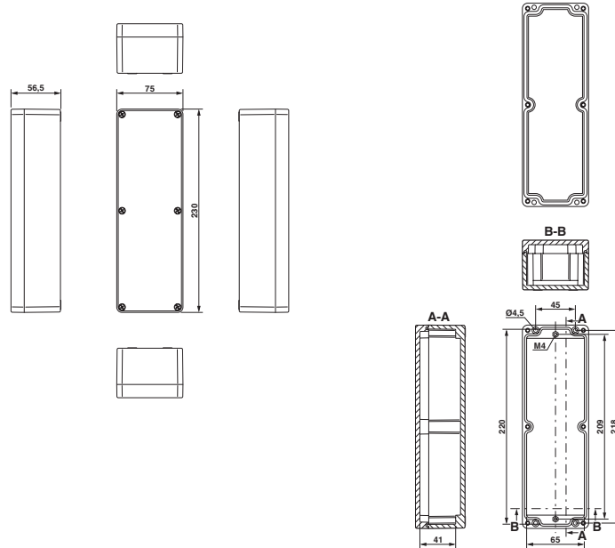
Schematic diagram
