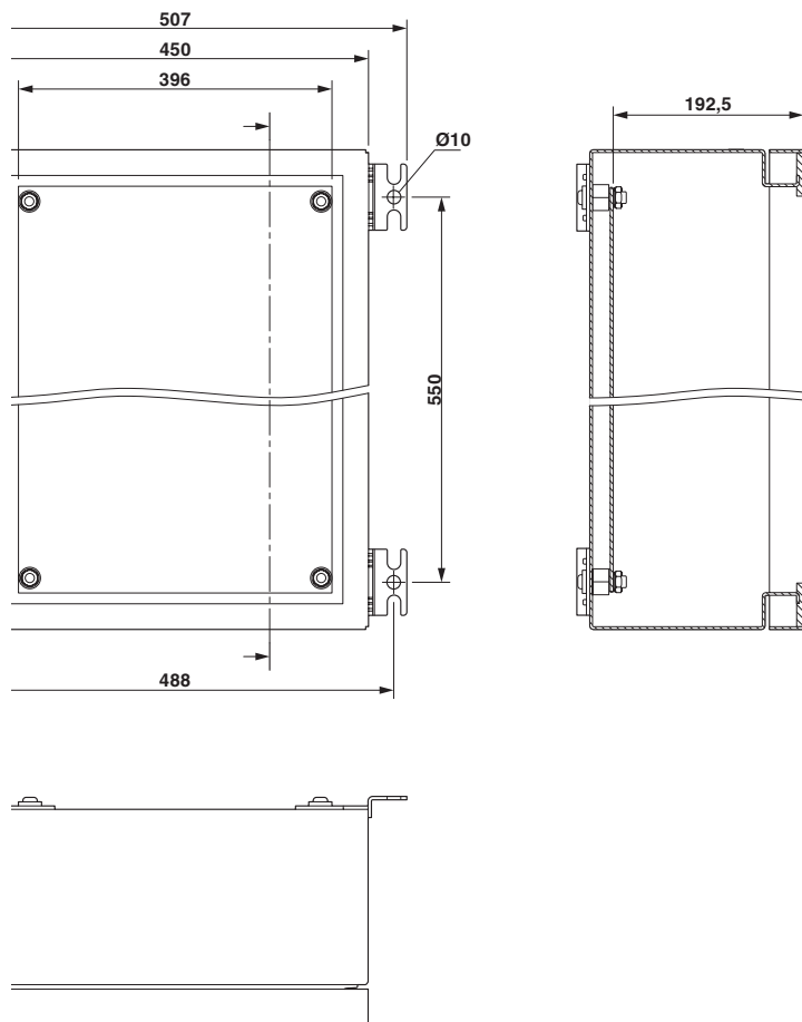
Dimensional drawing
