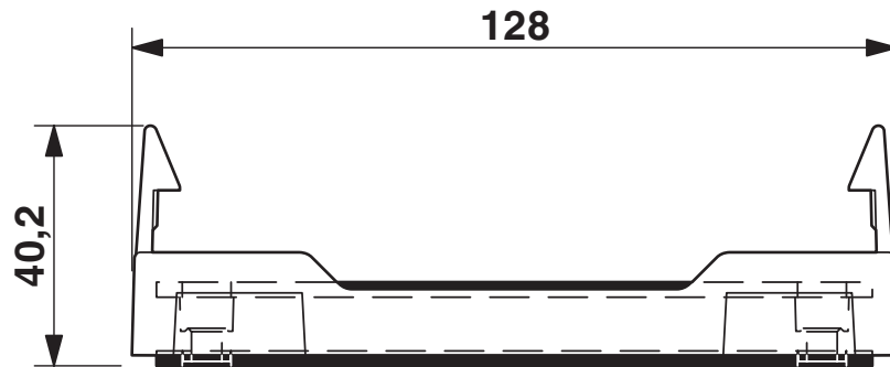
Dimensional drawing
