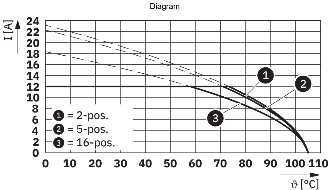
Type: FKCN 2,5/...-STF with DFK-MSTB 2,5/...-GF
