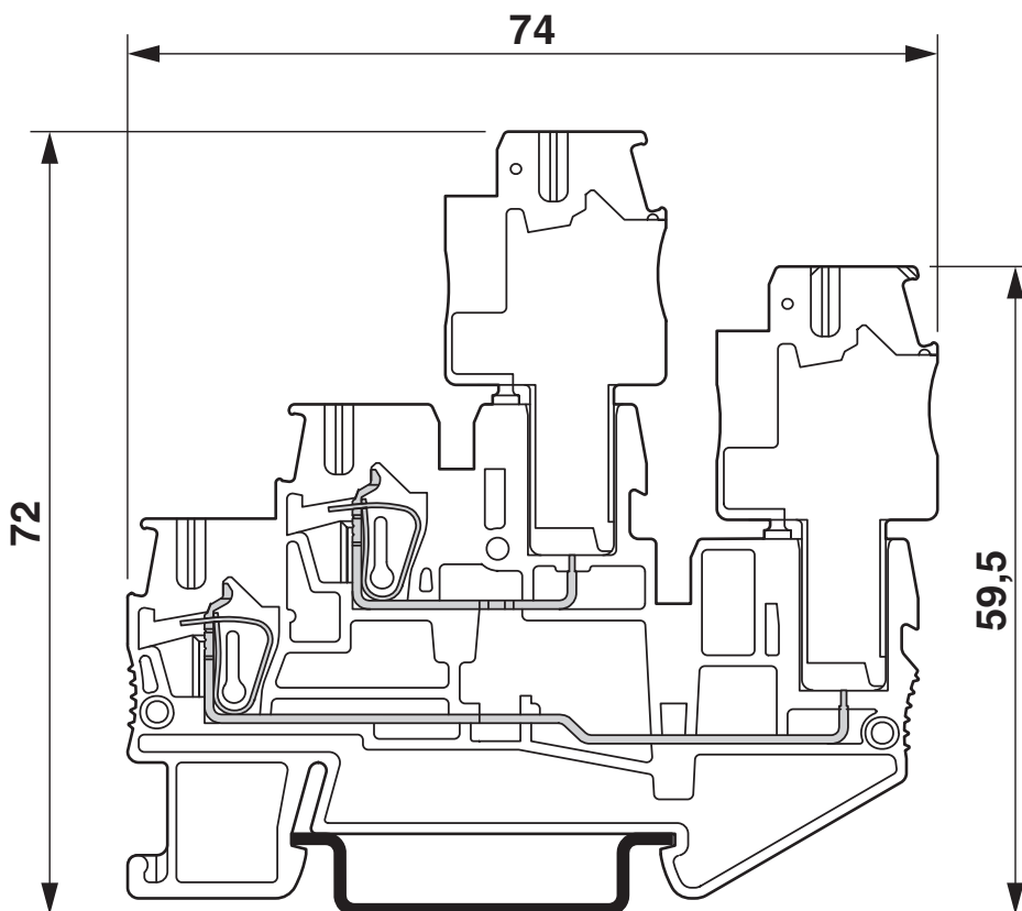
Dimensional drawing
