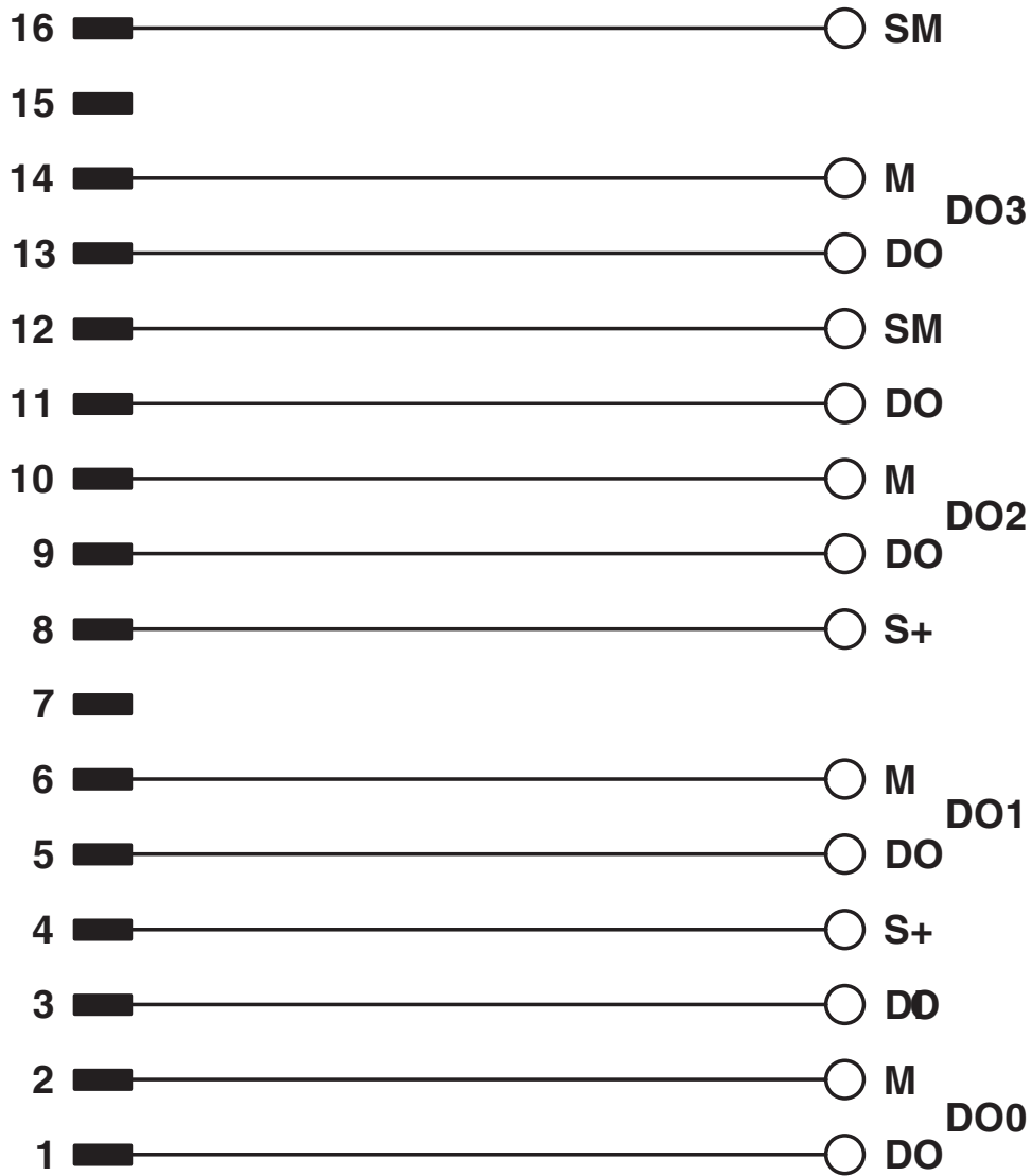
Circuit diagram
