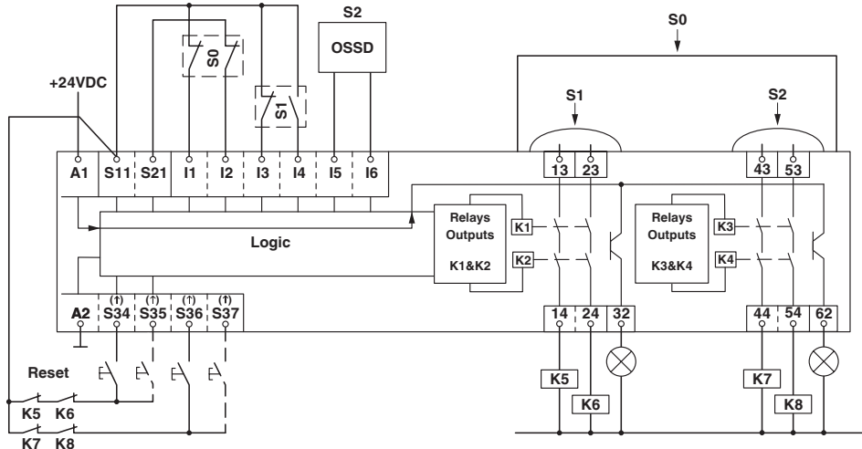
Circuit diagram
