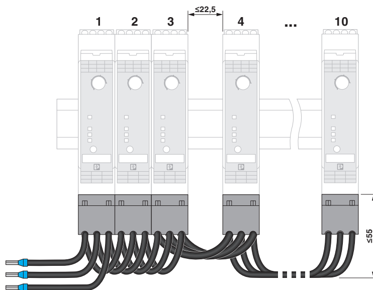
Application drawing
