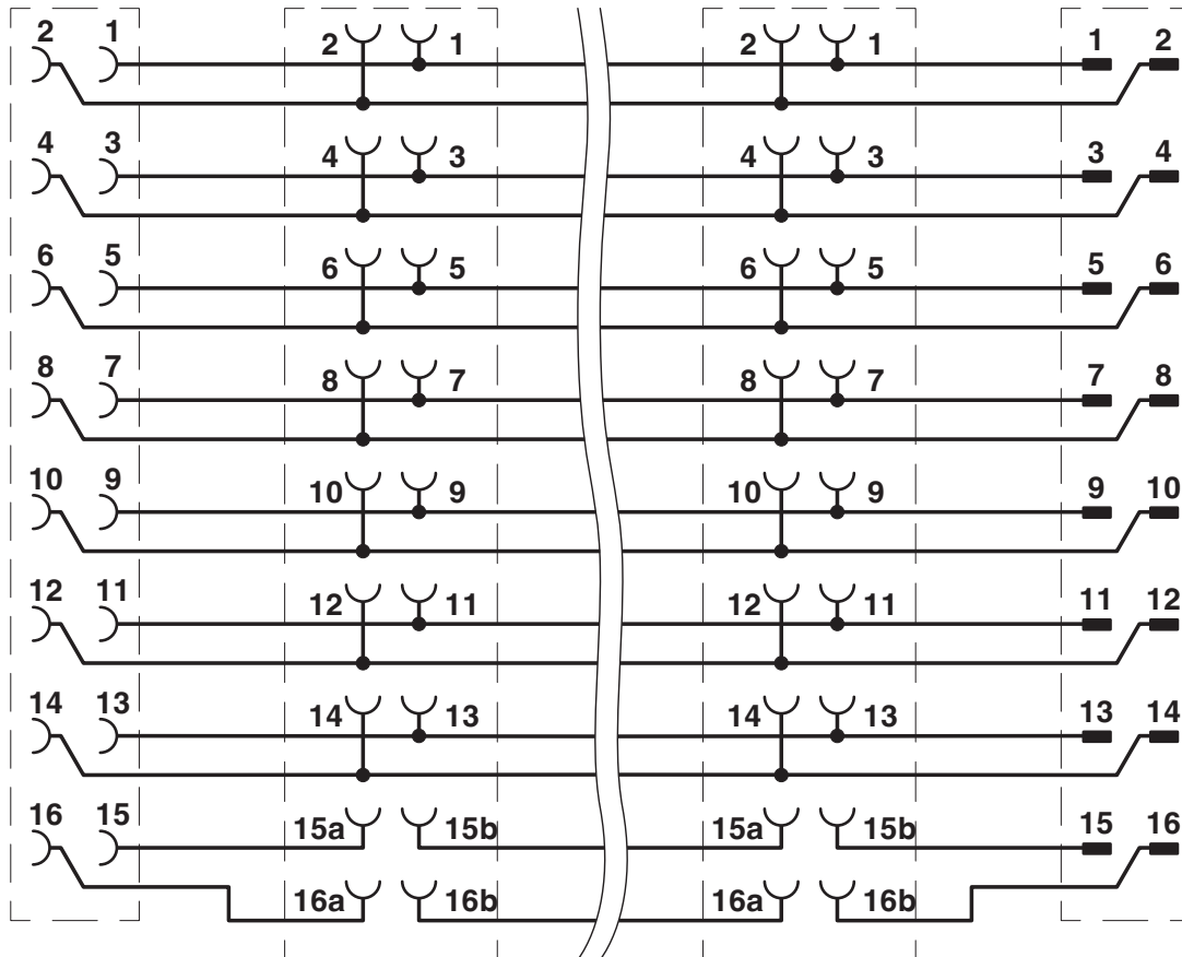
Circuit diagram
