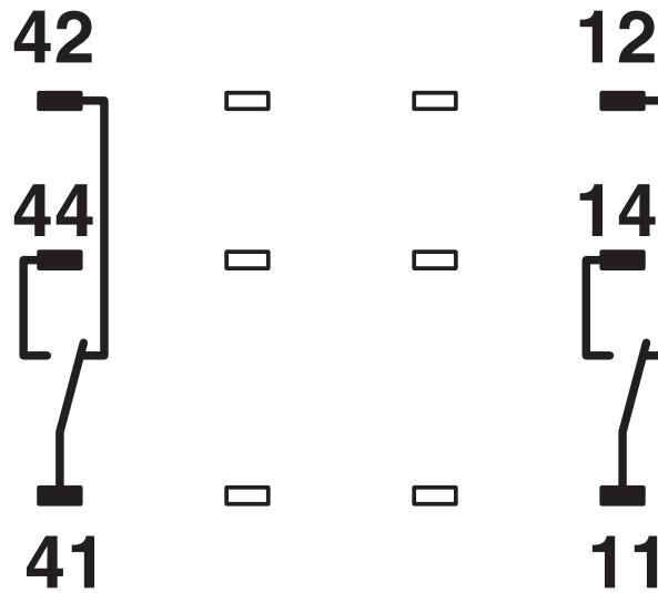
Circuit diagram
