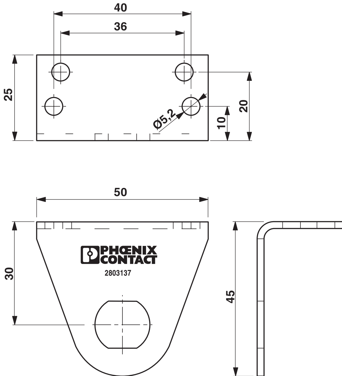
Dimensional drawing
