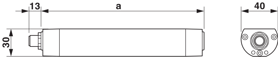
Dimensional drawing
