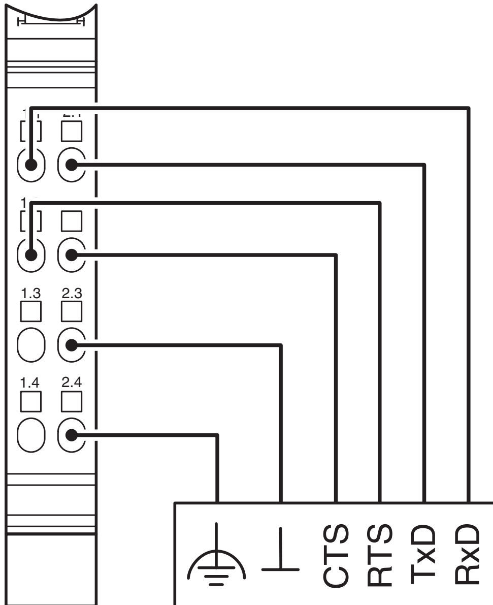
Connection diagram
