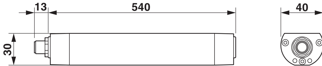
Dimensional drawing
