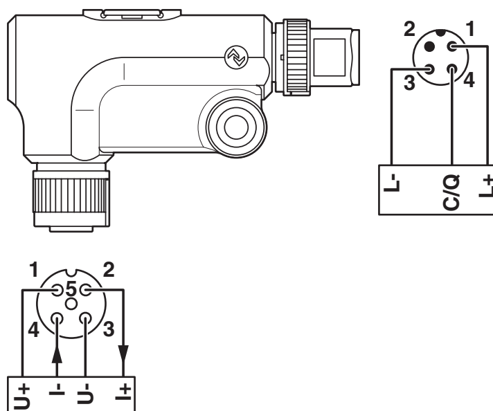
Connection diagram
